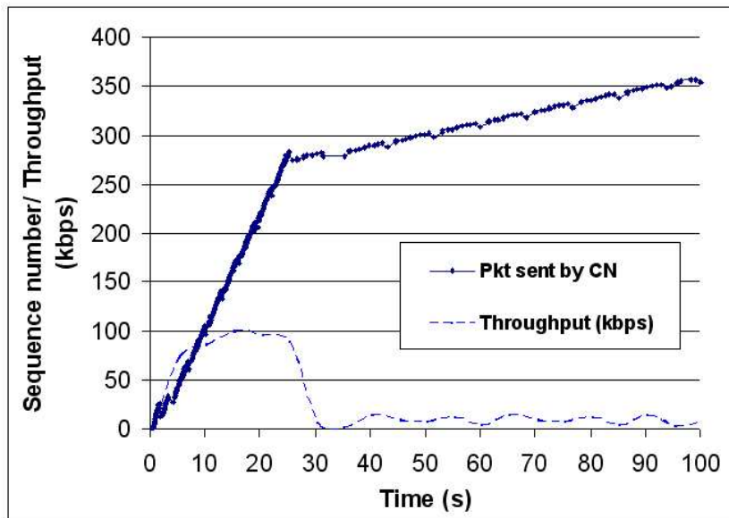
Figure 6.5: Progress in TCP packet sequence number at CN, and throughput observed by MN in general upward vertical handover (i.e., without graceful handover). The MN performed a handover after 25 seconds.
