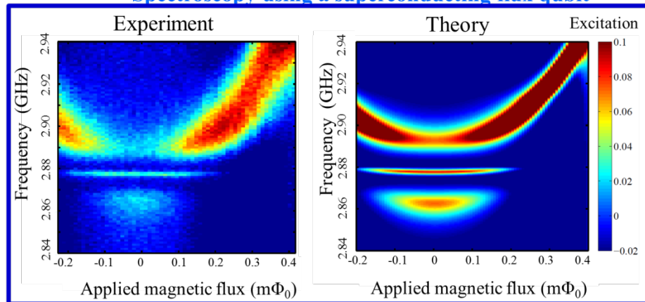
Fig.5 Spectroscopy using a superconducting flux qubit
