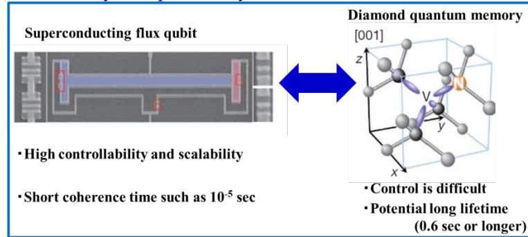
Fig. 1 Hybrid device to realize quantum computation
