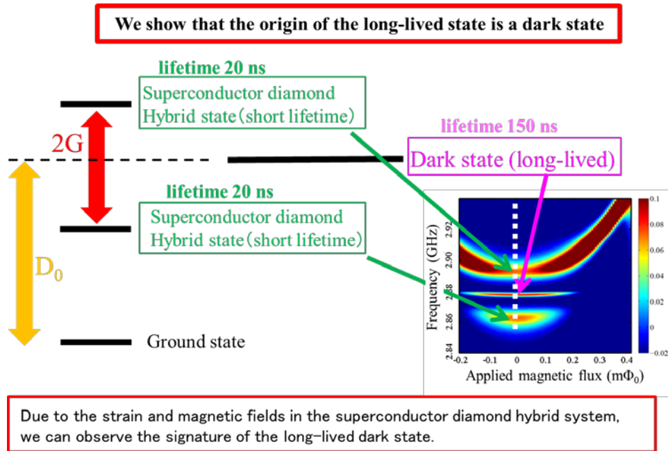
Fig. 3 The mechanism for the observation of a long-lived dark state
