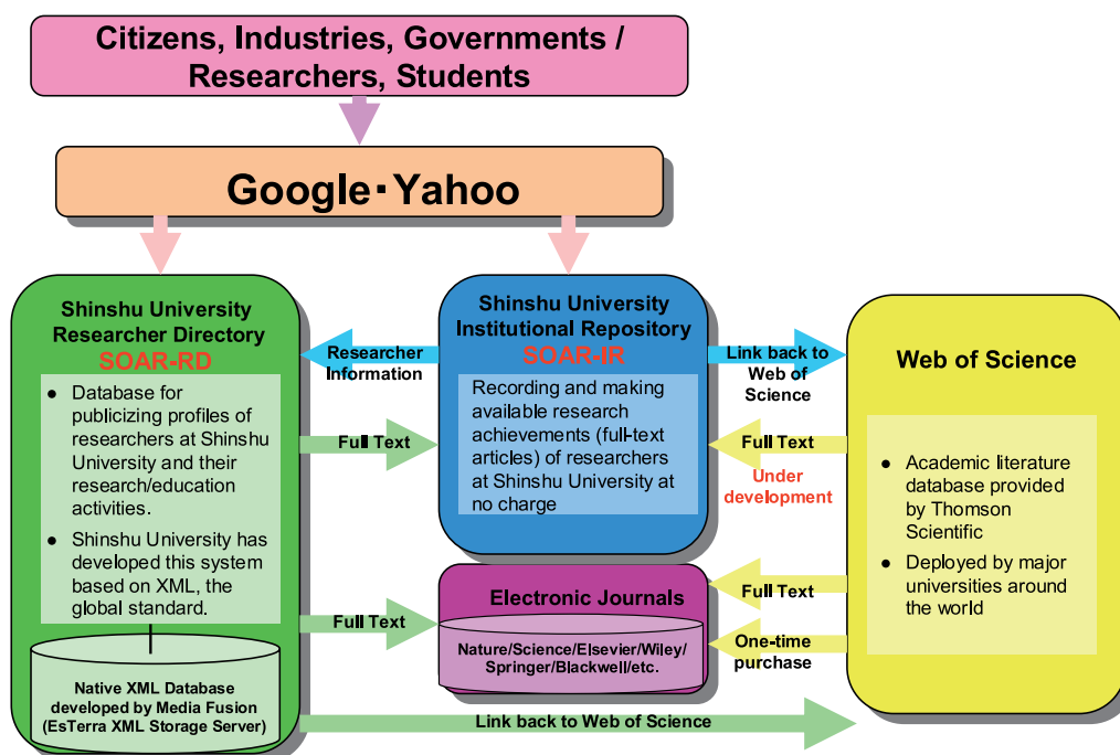
Fig. 1 SOAR overview.
